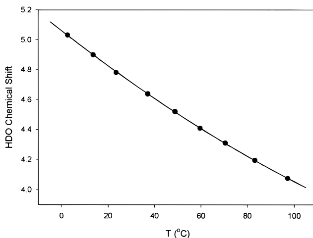
Figure 1. Chemical shift of \text{HDO} as a function of temperature.
